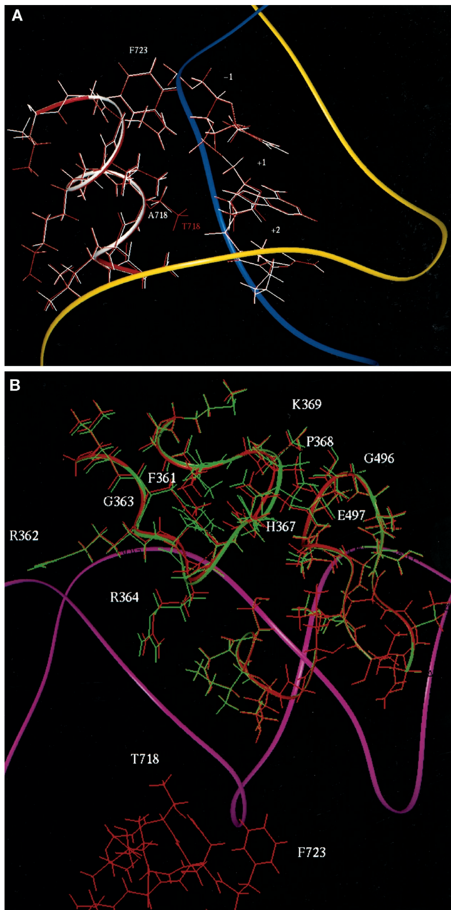
Fig. 9. A, minimized structures in the region of the Thr718 and the active site tyrosine. Superimposition of wild-type hTop1p (red) and hTop1T718Ap (Ala substituted for Thr-718) (white) structures after minimization. The yellow DNA ribbon indicates the nonscissile strand. B, minimized structures in the region of the Cpt-loop. Superimposition of the wild-type hTop1p (red) and Val substituted for Gly-363 (green).
