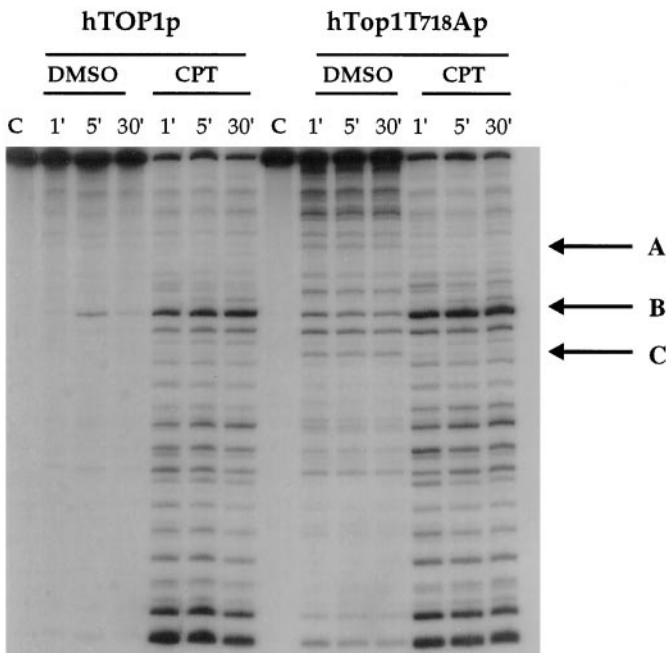
Fig. 5. hTop1T718Ap increases the stability of the covalent enzyme-DNA intermediate in the absence of Cpt. In vitro DNA cleavage activity of bead-bound epitope-tagged ehTop1p and ehTop1T718Ap was assayed. A 3' 32 P end-labeled DNA fragment was incubated with immunoprecipitated ehTop1p or ehTop1T718Ap for the times indicated, in the presence of 4% DMSO or 100 μM Cpt. Control, no enzyme added (C). Total protein (110 ng), with comparable specific activity, was used in each assay. Arrows A and C indicate cleavage sites mostly evident in the hTop1T718Ap in the absence of Cpt and arrow B indicates the preferred cleavage site derived from Tetrahymena rDNA.
