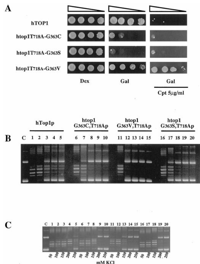
Fig. 7. Mutations at position 363 can suppress the lethality of htop1T718A . A, viability of EKY2 ( top1Δ ) cells transformed with the indicated YCpGAL1-hTOP1 construct. Five microliters of serial 10-fold dilutions of cultures starting from A_{595} = 0.5 , were spotted onto SC-uracil plates containing 2% dextrose or 2% galactose and 5 \mu g/ml Cpt. B, 1 \mu l of serial 5-fold dilutions of partially purified wild-type or mutant hTop1p were assayed for their ability to relax 0.5- \mu g supercoiled plasmid DNA. Lanes 1–5, hTop1p; lanes 6–10, hTop1G363C, T718Ap; lanes 11–15, hTop1G363V, T718Ap; lanes 16–20, hTop1G363S, T718Ap. Control (C), no protein added. Equivalent protein concentrations were verified by western blotting with an antibody specific for hTop1p. C, 1 \mu l of partially purified wild-type hTop1 (1–5) hTop1G363C, T718Ap (6–10) hTop1G363V, T718Ap (11–15), or hTop1G363S, T718Ap (16–20) were assayed for their ability to relax 0.5- \mu g supercoiled plasmid DNA in the presence of the KCl concentrations.
