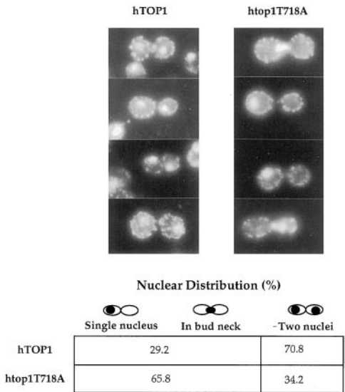
Fig. 6. Nuclear segregation is defective in strains overexpressing htop1T718A . EKY2 ( top1Δ ) cells were transformed with YCpGAL1- hTOP1 or YcpGAL1- htop1T718A , and hTop1p expression was galactose-induced for 6 h before cells were processed for microscopy. The table shows the percentage of large-budded cells displaying a single or double nucleus. Scoring was done by an observer blinded to the identity of the samples.
