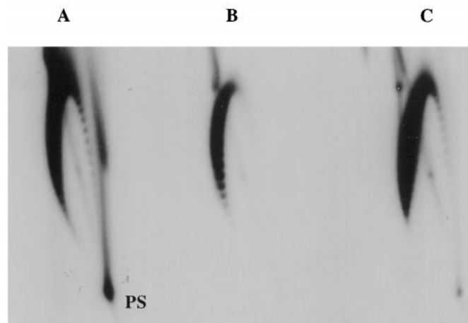
Fig. 4. hTop1T718A is active in vivo. Relaxation of positively supercoiled yeast 2- \mu m plasmid DNA by hTop1p and htop1T718Ap were assayed in vivo. Strain JCW28 ( top1Δ , top2-4 ) constitutively expressing a plasmid-borne Escherichia coli topA gene encoding bacterial DNA topoisomerase I, was transformed with a control plasmid YCpGAL1 (A), YCpGAL1-htop1T718A (B), or YCpGAL1-hTOP1 (C). Cultures were incubated at 25°C, a permissive temperature for JCW28 strain, and induced with galactose. Cultures were then shifted to 37°C to inactivate yeast DNA topoisomerase II. The 2- \mu m plasmid DNA was recovered from each culture after the temperature shift and analyzed in southern blots of two-dimensional agarose gels electrophoresis. PS, positive supercoils.
